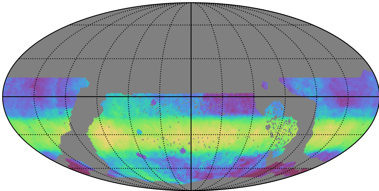
too_5_1v3.4_10yrs WFD i band: Median HA
