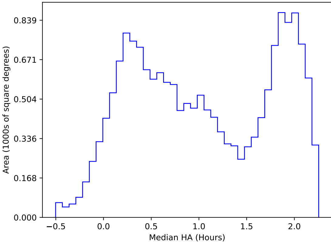
too_5_1v3.4_10yrs WFD i band: Median HA
