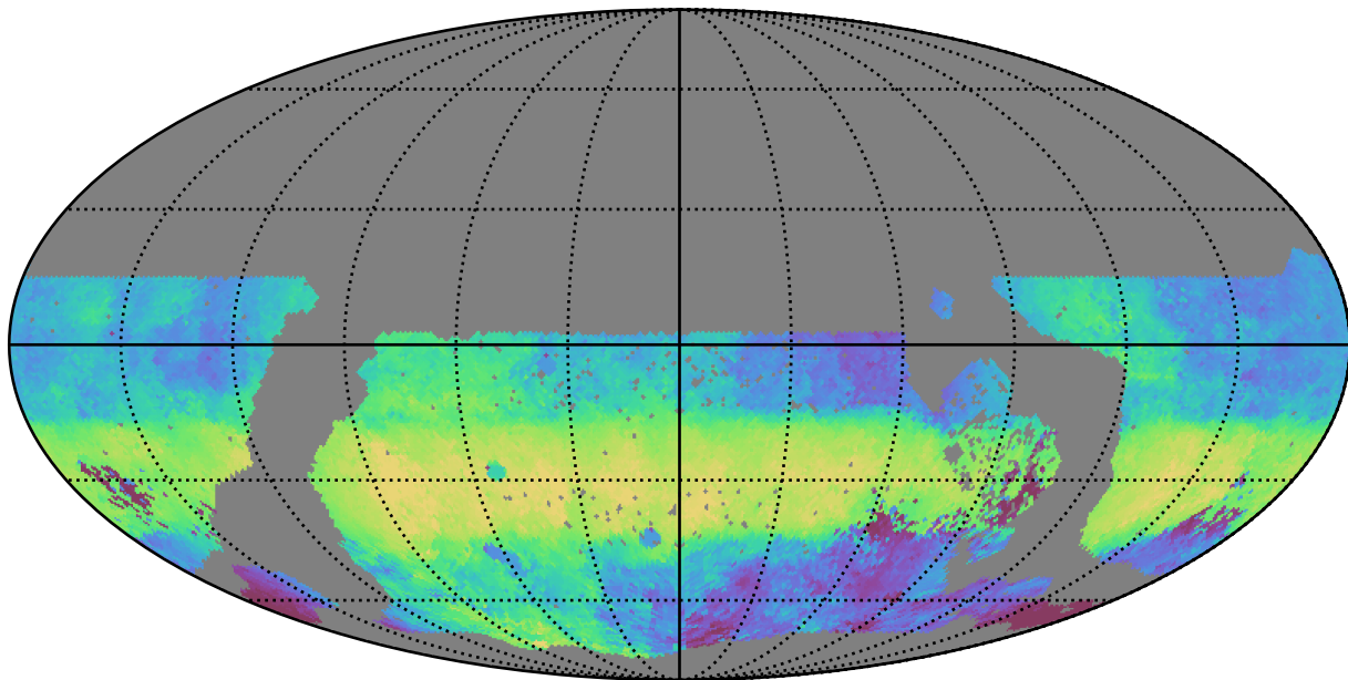
too_5_1v3.4_10yrs WFD g band: Median HA
