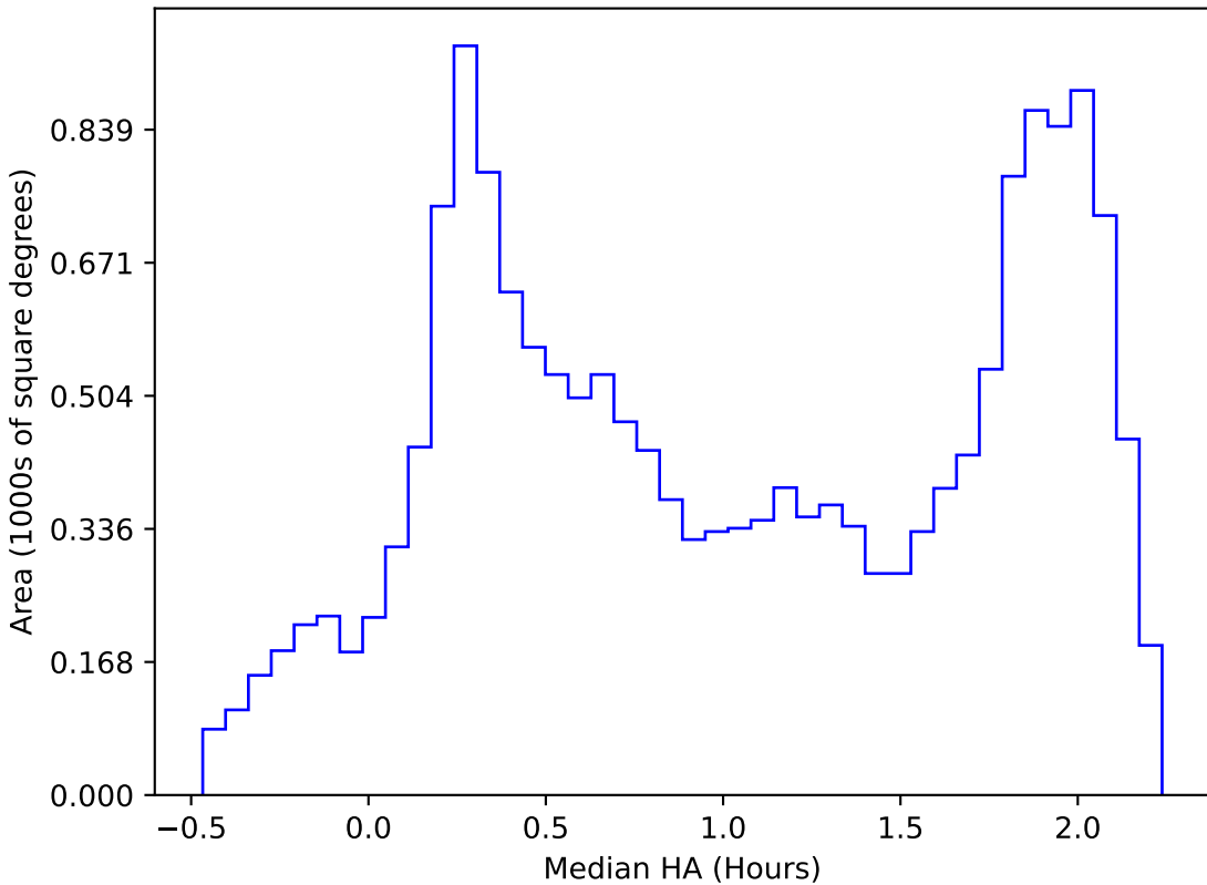
too_5_1v3.4_10yrs WFD all bands: Median HA
