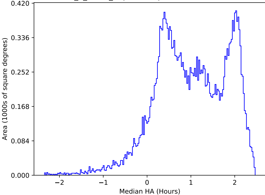
too_5_1v3.4_10yrs All sky z band: Median HA
