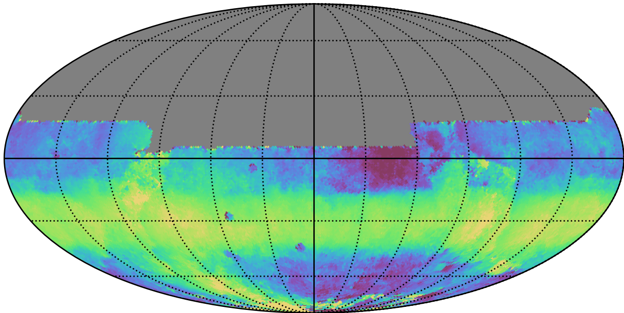
too_5_1v3.4_10yrs All sky y band: Median HA
