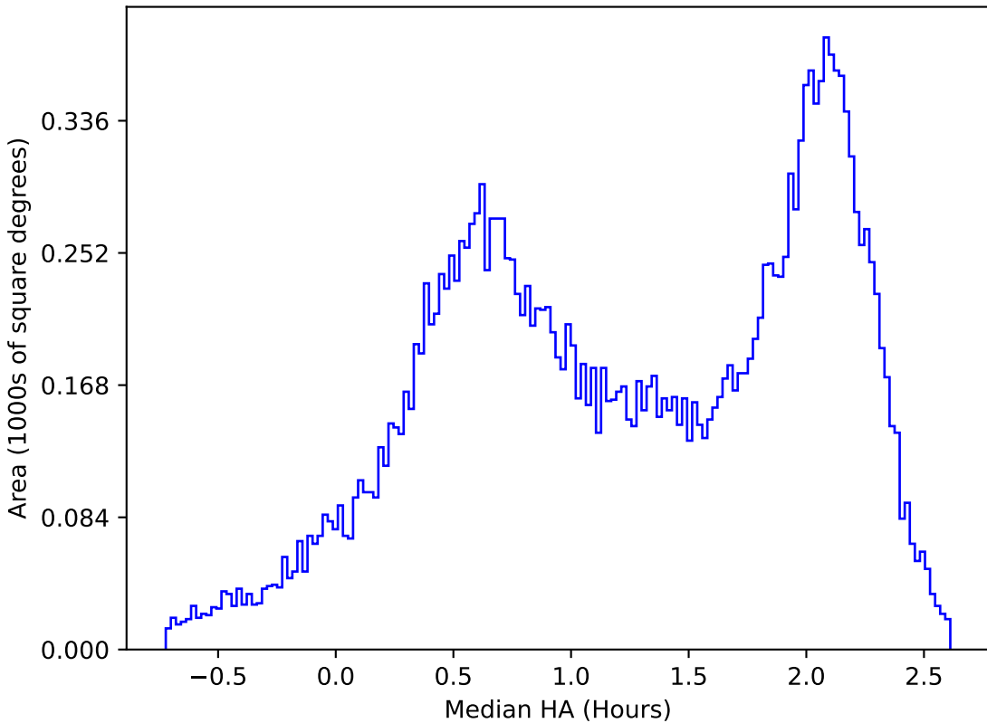
too_5_1v3.4_10yrs All sky y band: Median HA
