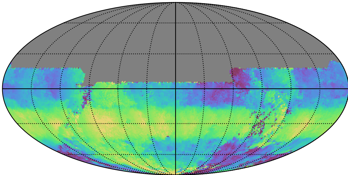
too_5_1v3.4_10yrs All sky u band: Median HA
