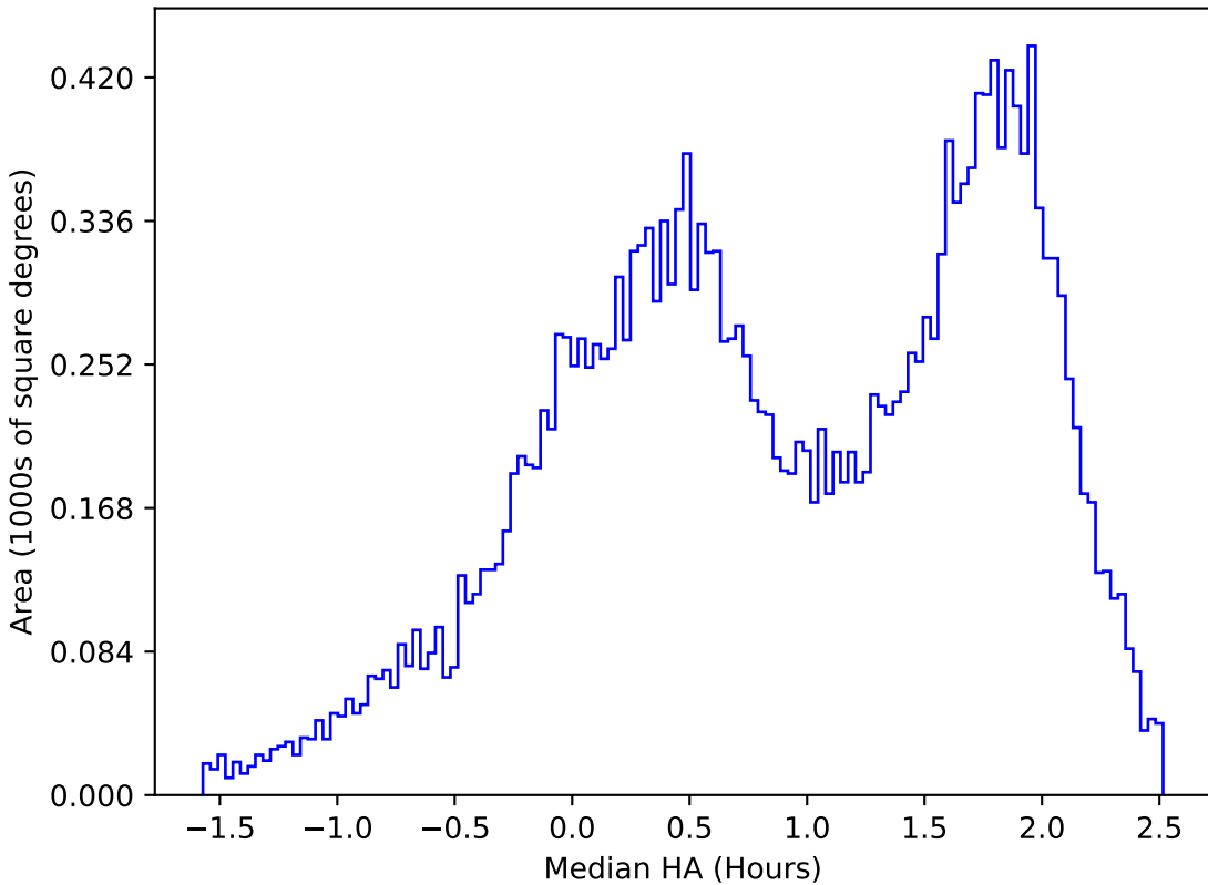
too_5_1v3.4_10yrs All sky u band: Median HA
