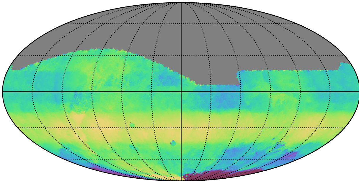
too_5_1v3.4_10yrs All sky r band: Median HA
