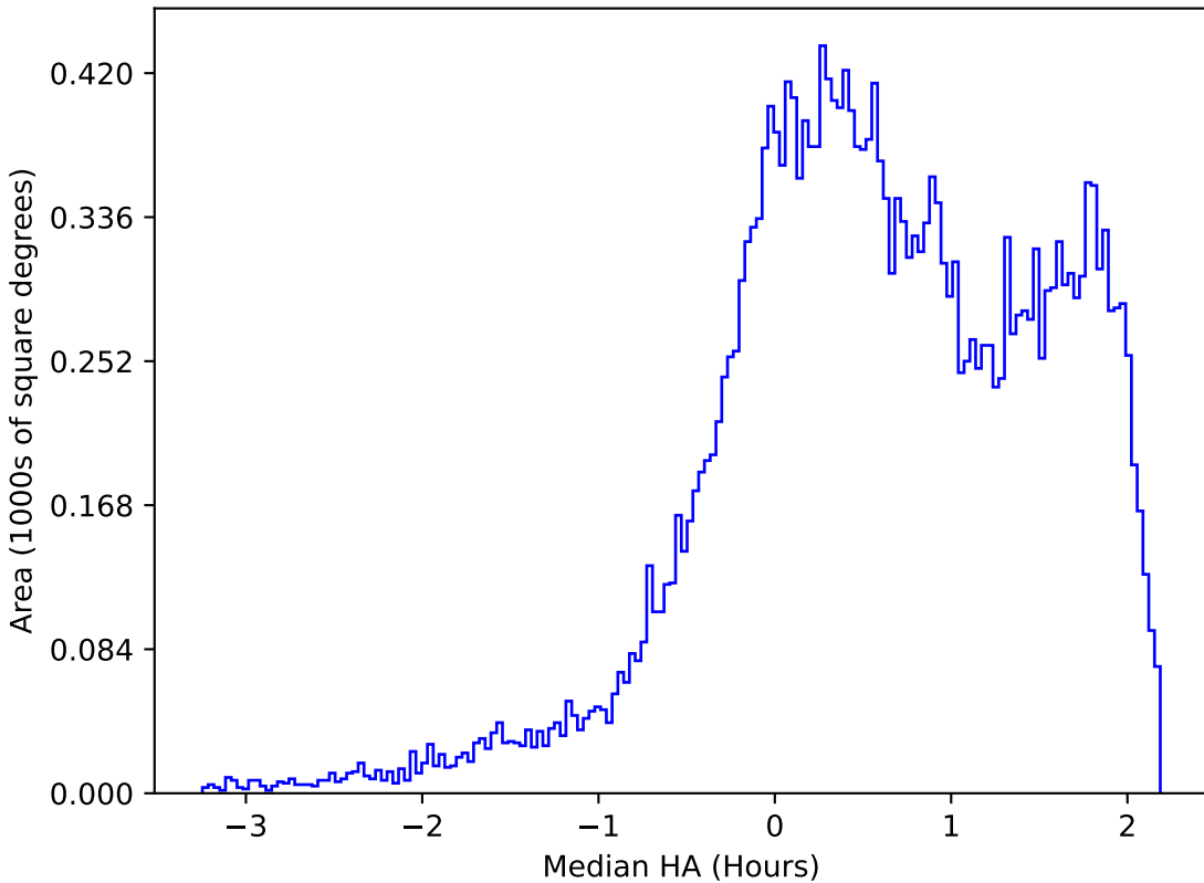
too_5_1v3.4_10yrs All sky g band: Median HA
