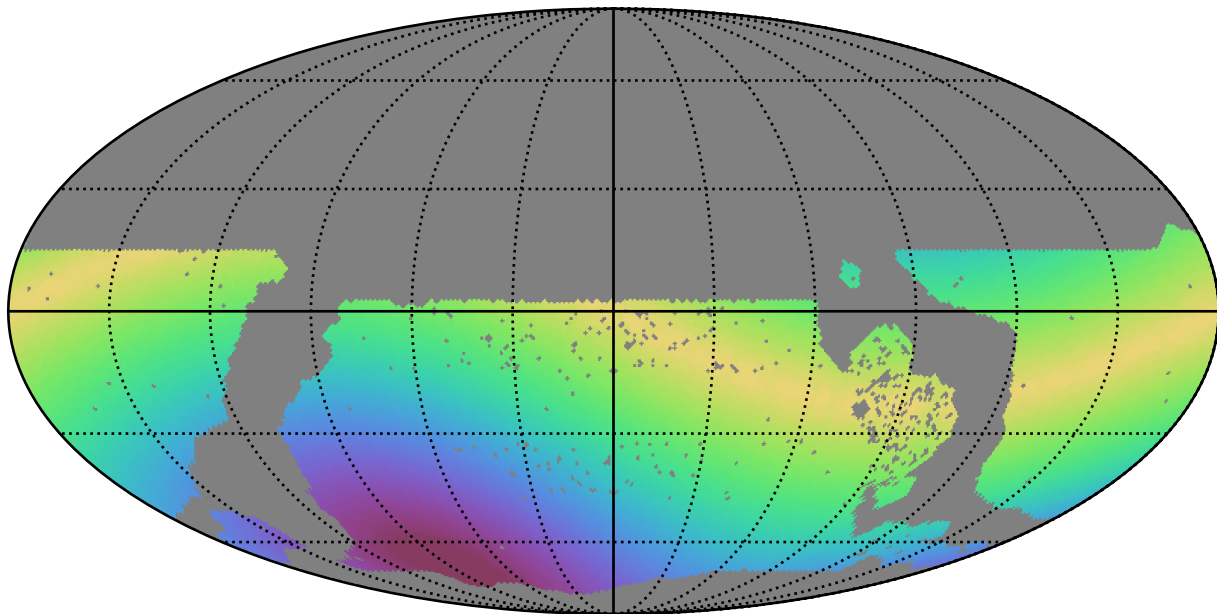
too_5_1v3.4_10yrs WFD z band: Max solarElong
