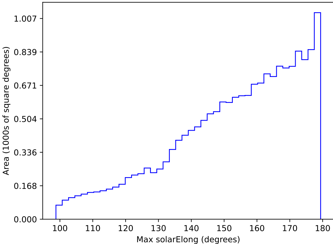
too_5_1v3.4_10yrs WFD z band: Max solarElong
