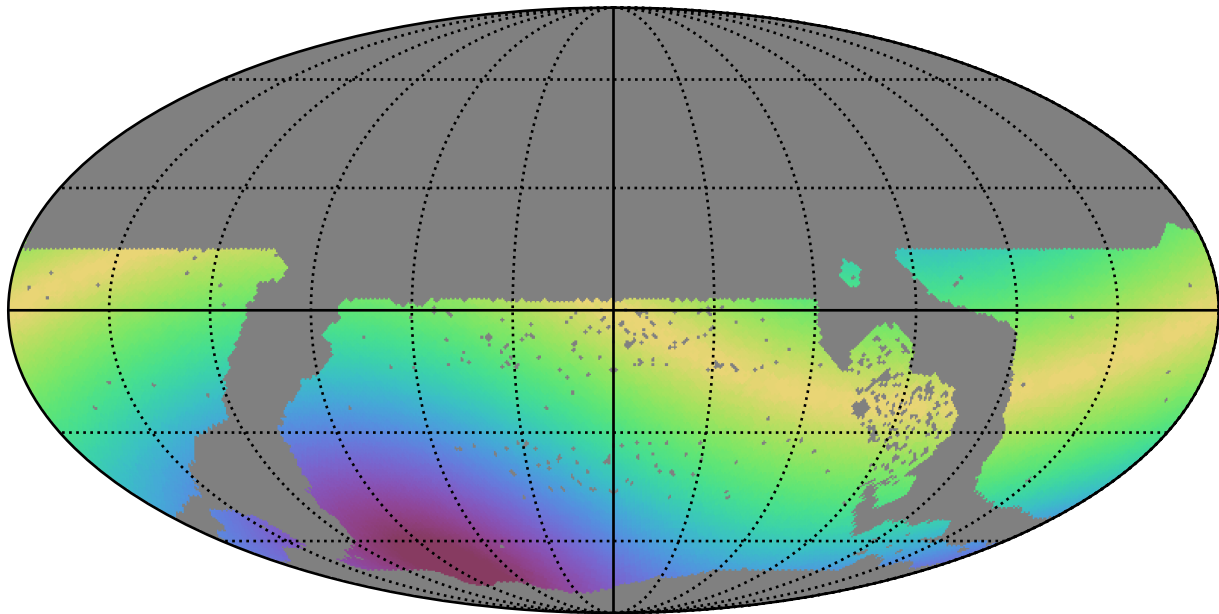
too_5_1v3.4_10yrs WFD r band: Max solarElong
