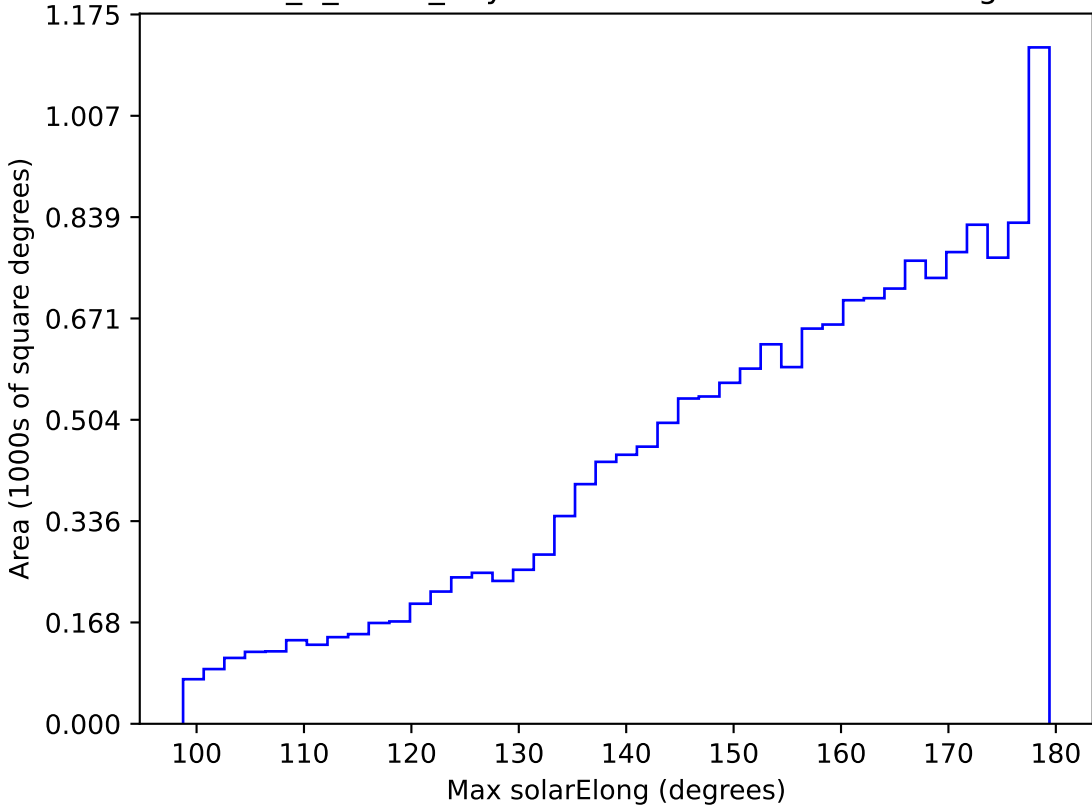
too_5_1v3.4_10yrs WFD r band: Max solarElong
