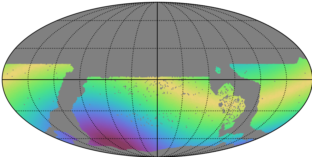
too_5_1v3.4_10yrs WFD i band: Max solarElong
