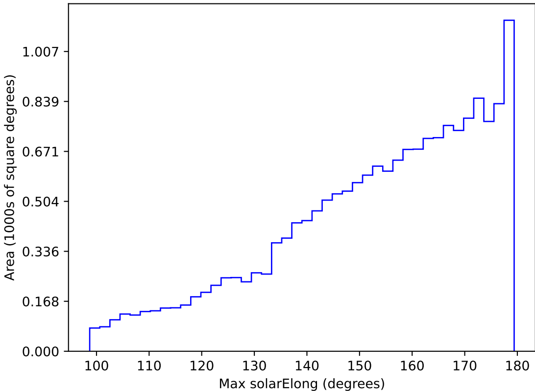
too_5_1v3.4_10yrs WFD i band: Max solarElong
