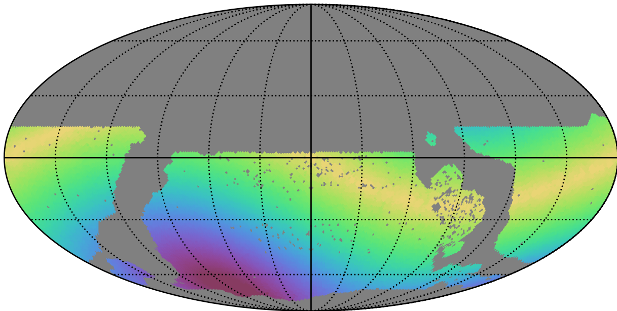
too_5_1v3.4_10yrs WFD g band: Max solarElong
