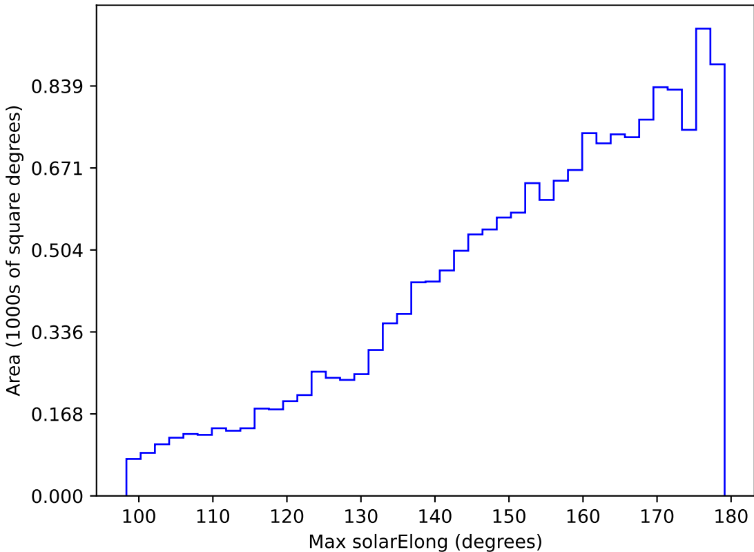
too_5_1v3.4_10yrs WFD g band: Max solarElong
