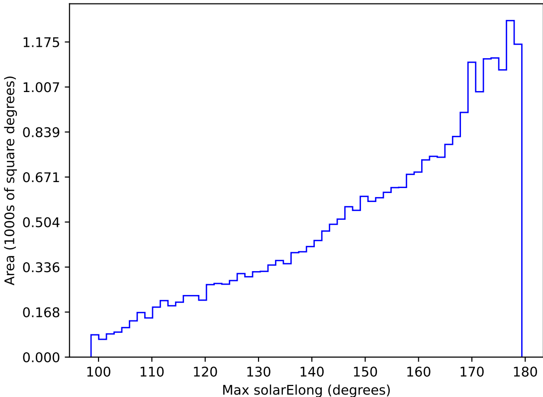
too_5_1v3.4_10yrs All sky z band: Max solarElong
