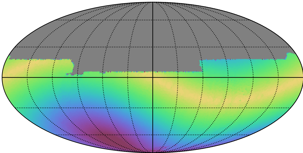
too_5_1v3.4_10yrs All sky y band: Max solarElong
