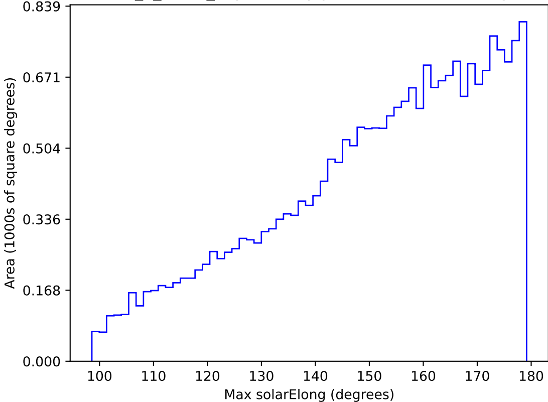
too_5_1v3.4_10yrs All sky y band: Max solarElong
