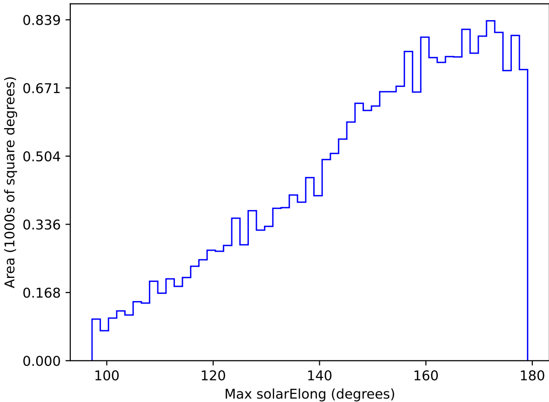
too_5_1v3.4_10yrs All sky u band: Max solarElong
