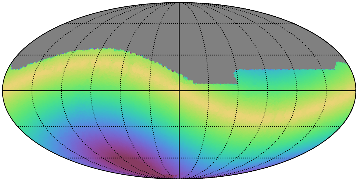
too_5_1v3.4_10yrs All sky r band: Max solarElong
