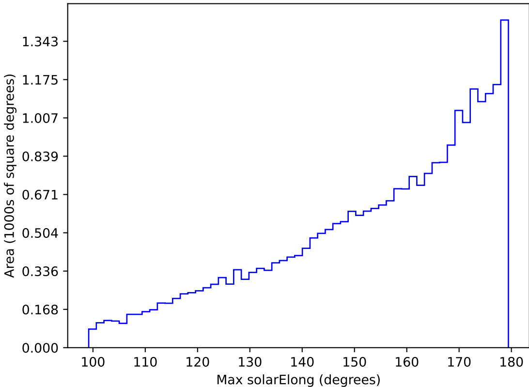
too_5_1v3.4_10yrs All sky r band: Max solarElong
