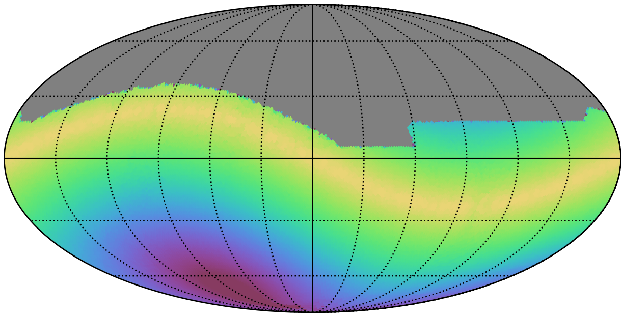
too_5_1v3.4_10yrs All sky i band: Max solarElong
