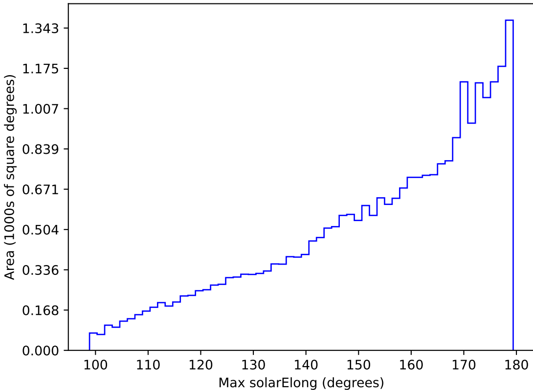
too_5_1v3.4_10yrs All sky i band: Max solarElong
