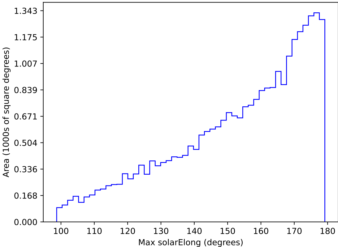
too_5_1v3.4_10yrs All sky g band: Max solarElong
