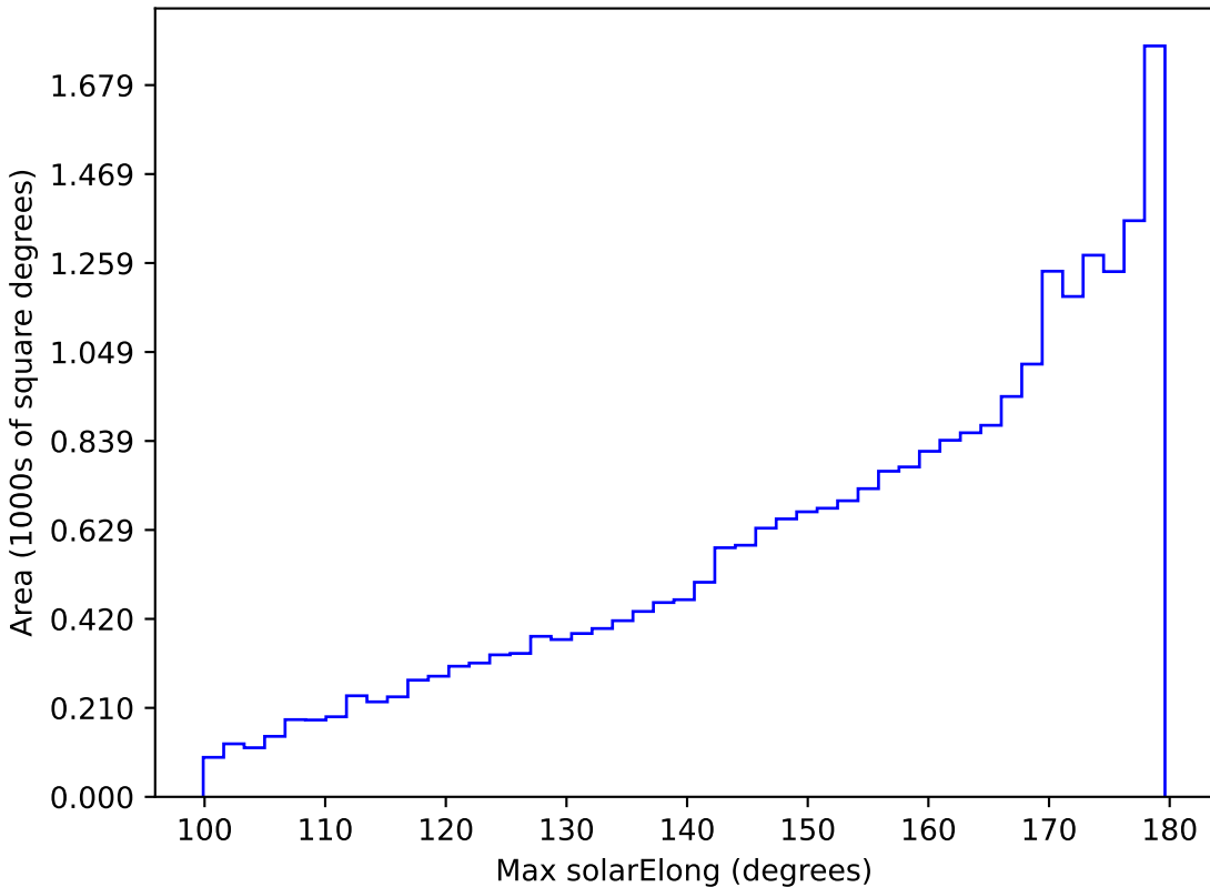
too_5_1v3.4_10yrs All sky all bands: Max solarElong
