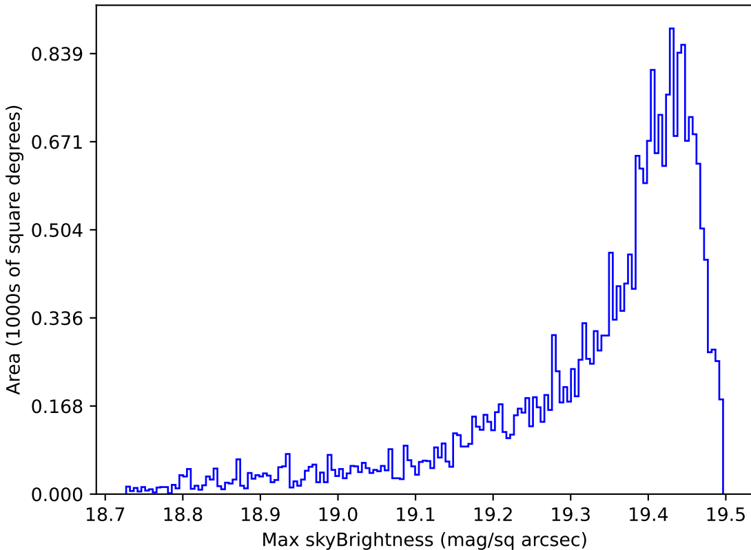
too_5_1v3.4_10yrs Yr 1 z band: Max skyBrightness
