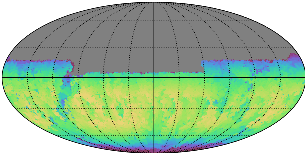
too_5_1v3.4_10yrs Yr 1 y band: Max skyBrightness
