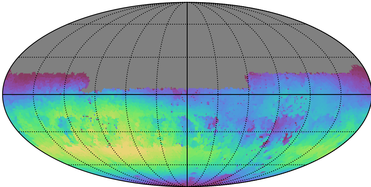
too_5_1v3.4_10yrs Yr 1 u band: Max skyBrightness
