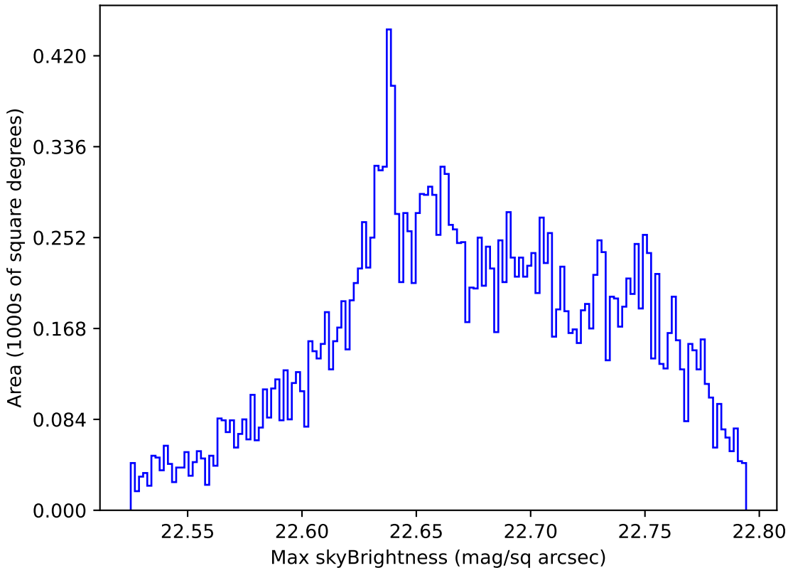
too_5_1v3.4_10yrs Yr 1 u band: Max skyBrightness
