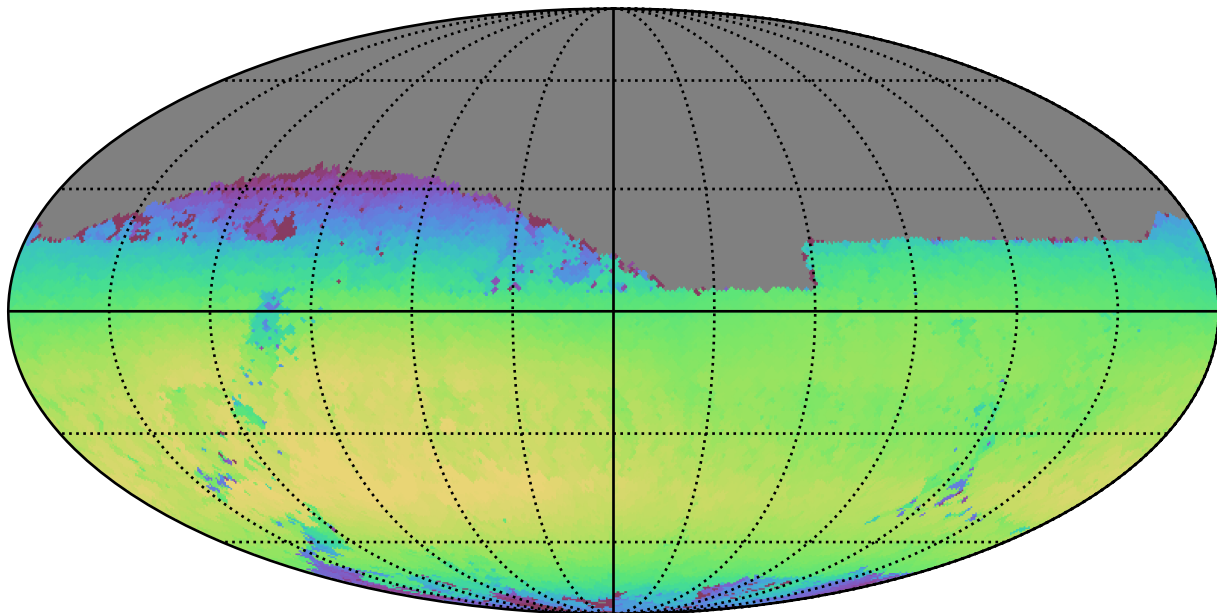
too_5_1v3.4_10yrs Yr 1 i band: Max skyBrightness
