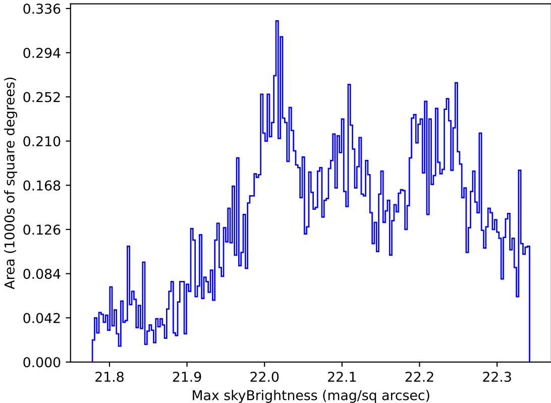
too_5_1v3.4_10yrs Yr 1 g band: Max skyBrightness
