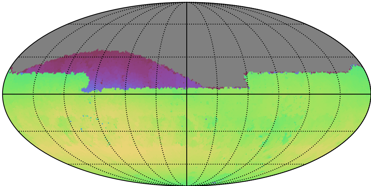
too_5_1v3.4_10yrs Yr 1 all bands: Max skyBrightness
