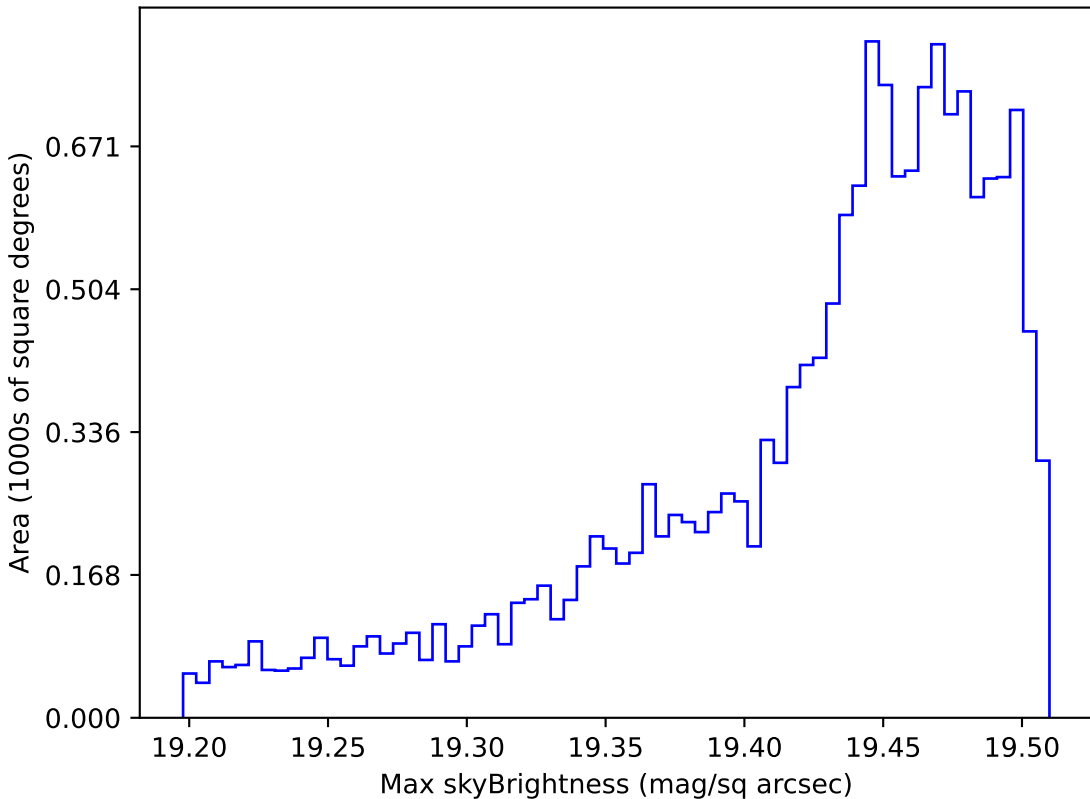
too_5_1v3.4_10yrs WFD z band: Max skyBrightness
