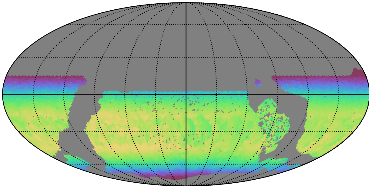
too_5_1v3.4_10yrs WFD y band: Max skyBrightness
