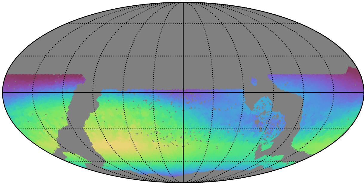
too_5_1v3.4_10yrs WFD u band: Max skyBrightness
