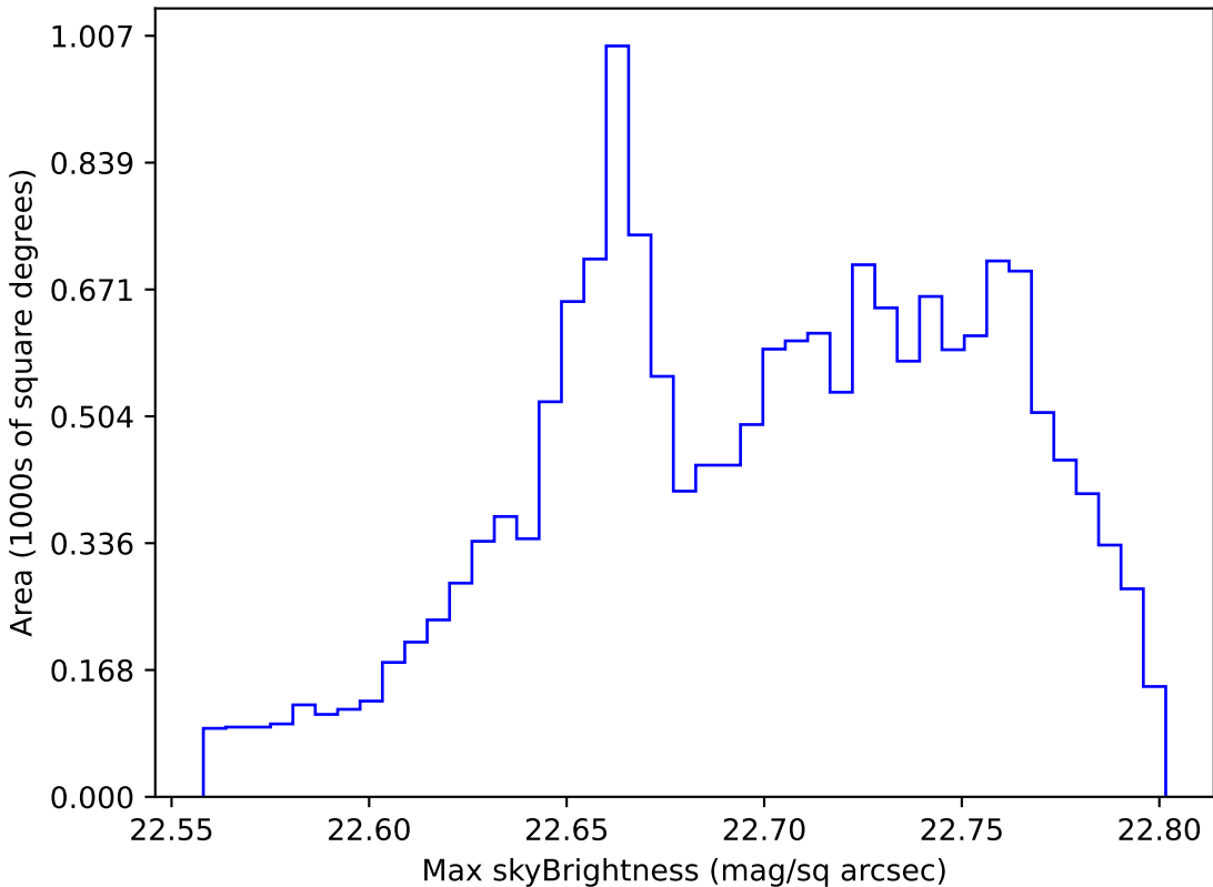
too_5_1v3.4_10yrs WFD u band: Max skyBrightness
