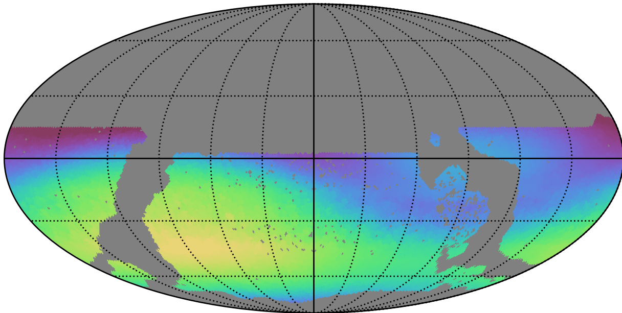
too_5_1v3.4_10yrs WFD r band: Max skyBrightness
