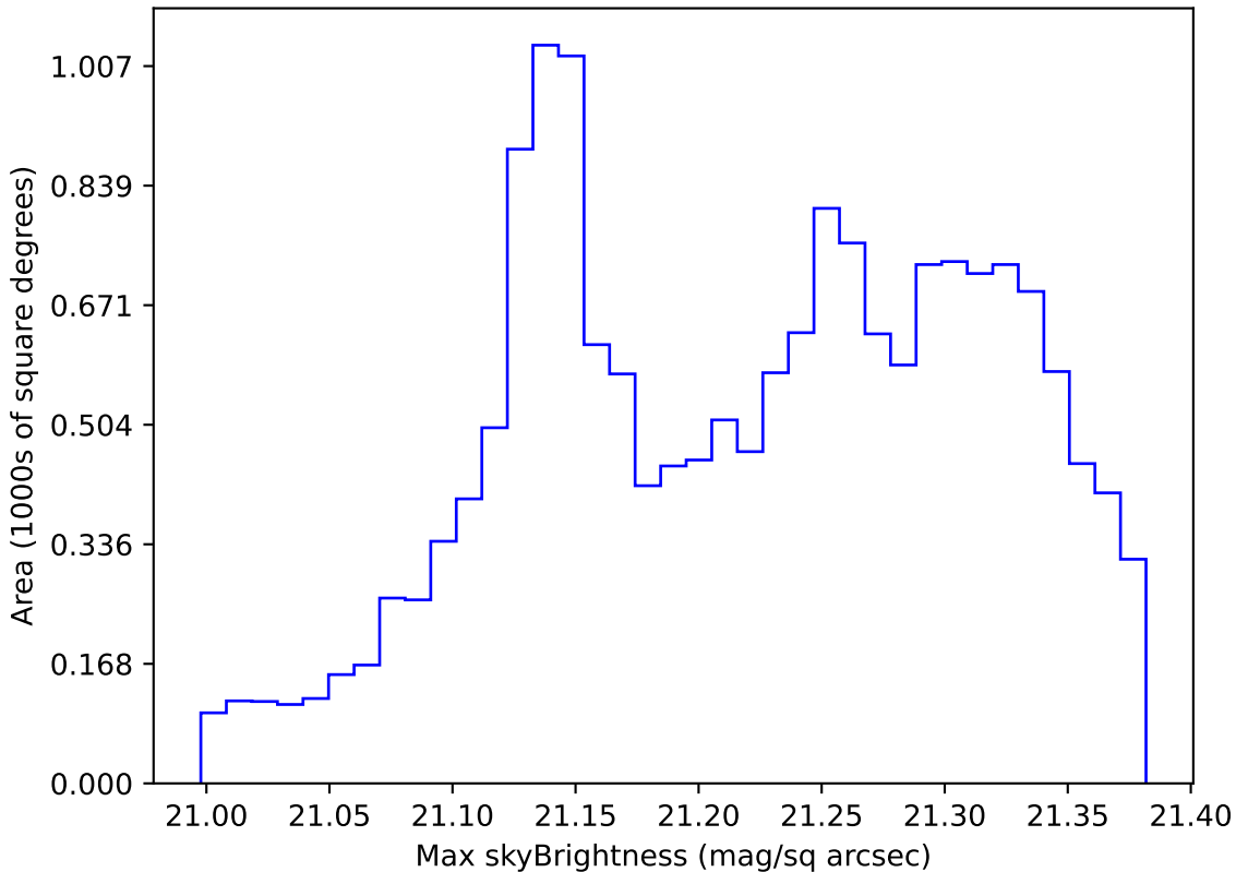
too_5_1v3.4_10yrs WFD r band: Max skyBrightness
