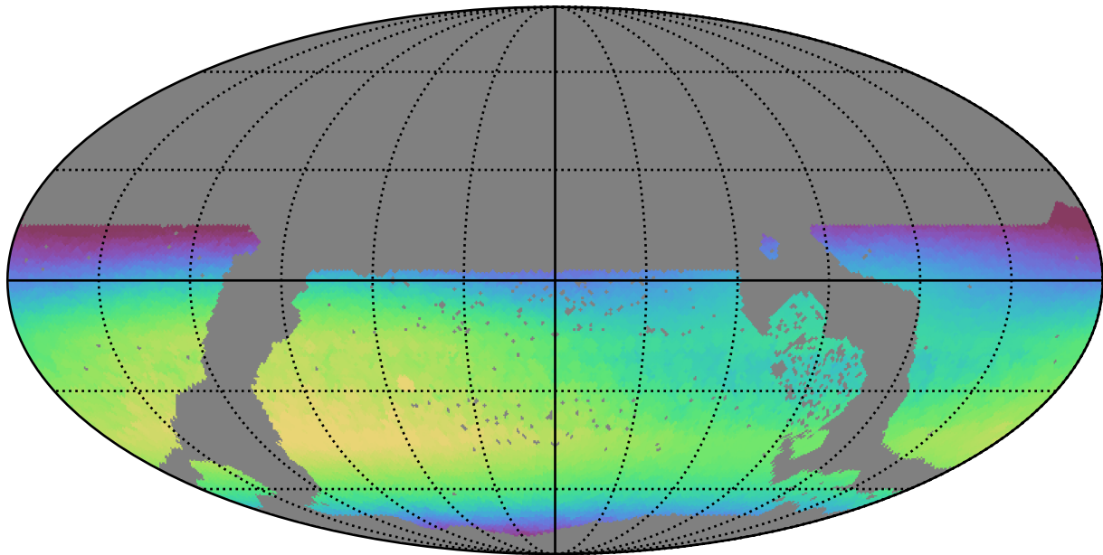
too_5_1v3.4_10yrs WFD i band: Max skyBrightness
