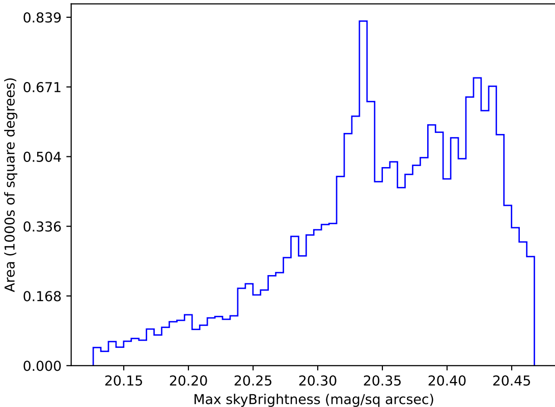
too_5_1v3.4_10yrs WFD i band: Max skyBrightness
