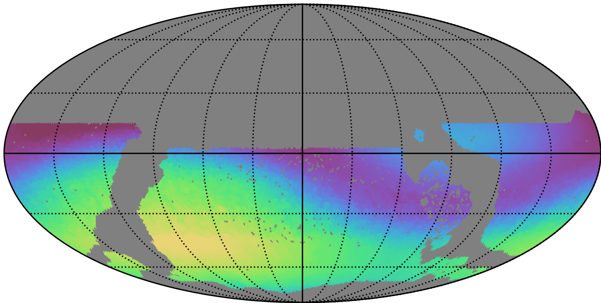
too_5_1v3.4_10yrs WFD g band: Max skyBrightness
