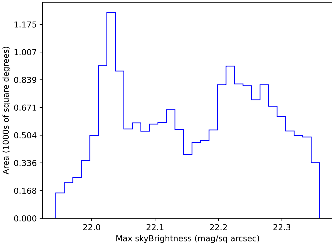
too_5_1v3.4_10yrs WFD g band: Max skyBrightness
