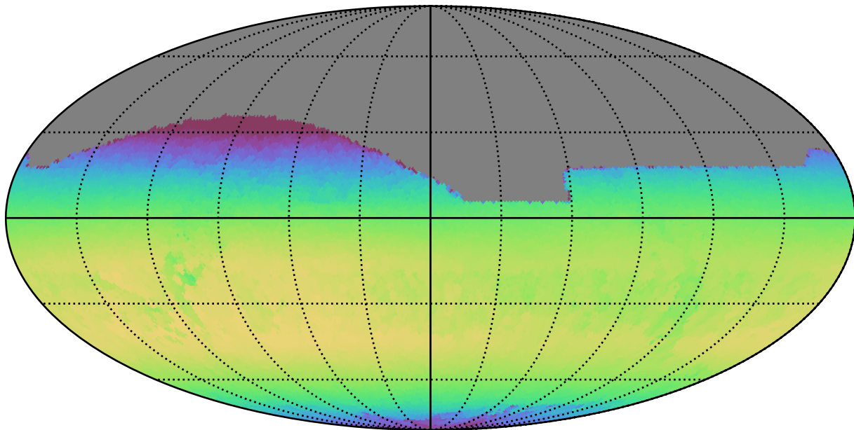
too_5_1v3.4_10yrs All sky z band: Max skyBrightness
