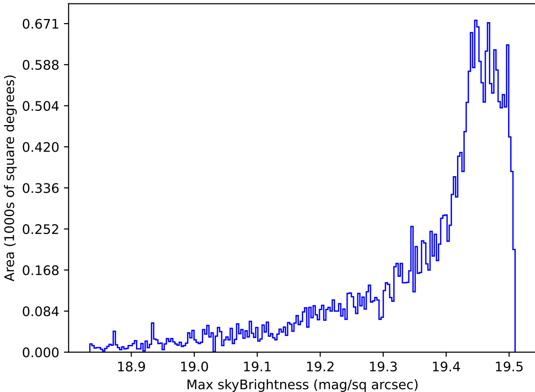
too_5_1v3.4_10yrs All sky z band: Max skyBrightness
