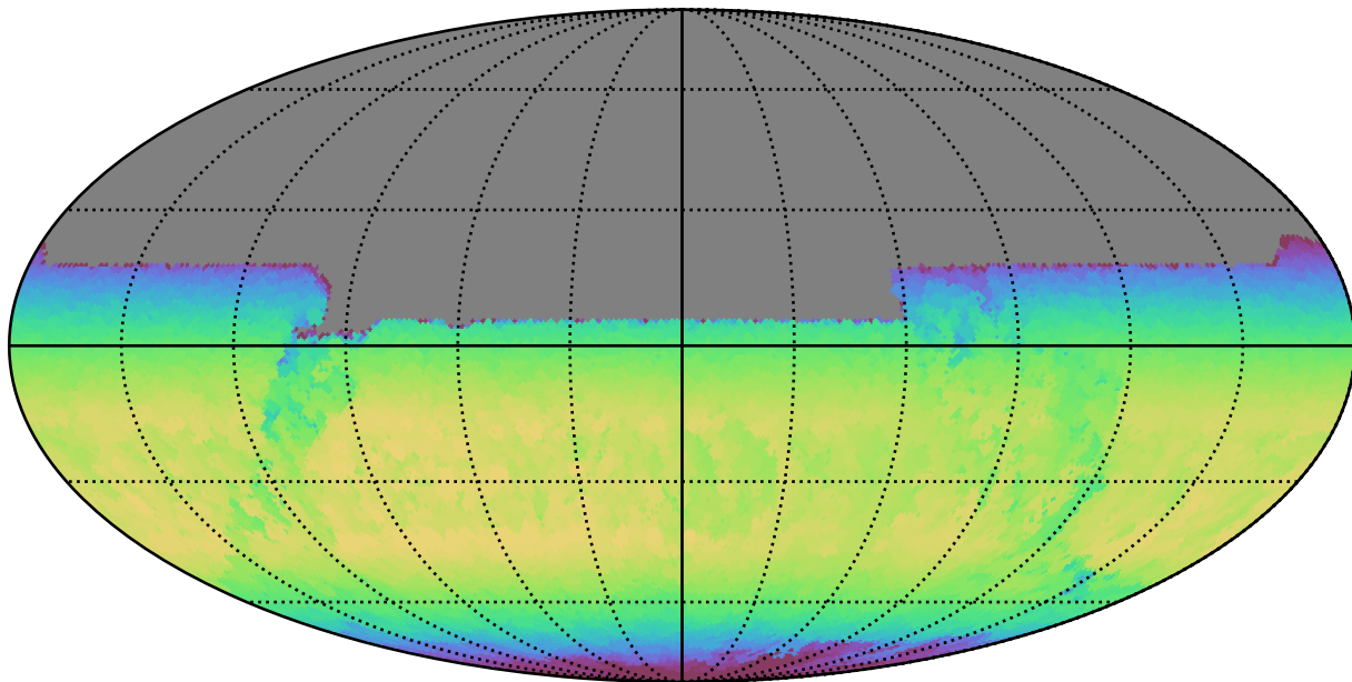
too_5_1v3.4_10yrs All sky y band: Max skyBrightness
