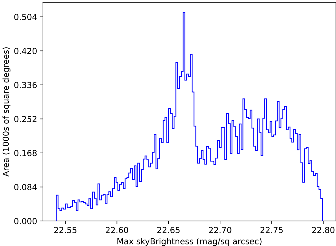
too_5_1v3.4_10yrs All sky u band: Max skyBrightness
